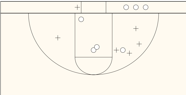
Scoring Distribution
