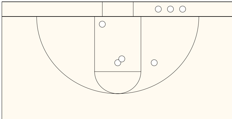
Scoring Locations
